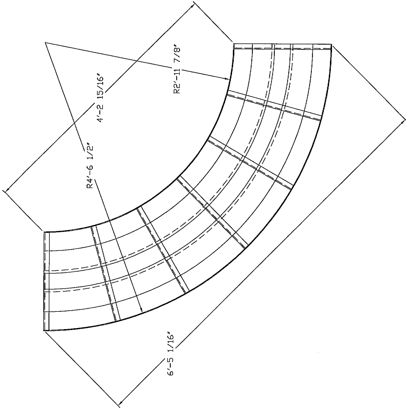
C121241-X92 RADIUS ROLL DETAIL
