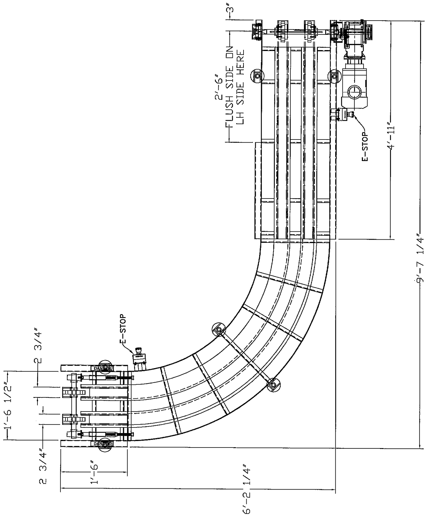
C121241-X92 PLAN VIEW
